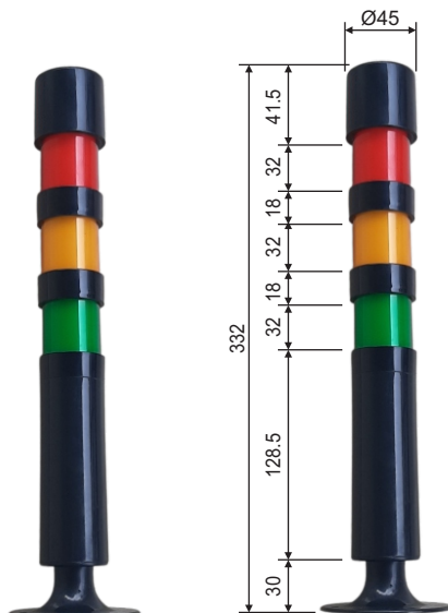
Base Mounting
