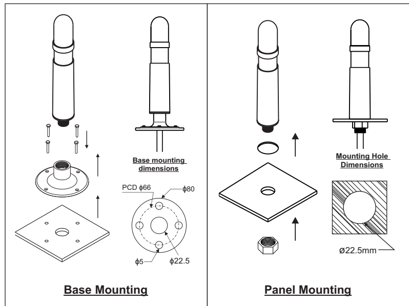
Mounting Dimensions
