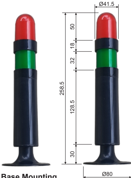
Base Mounting
