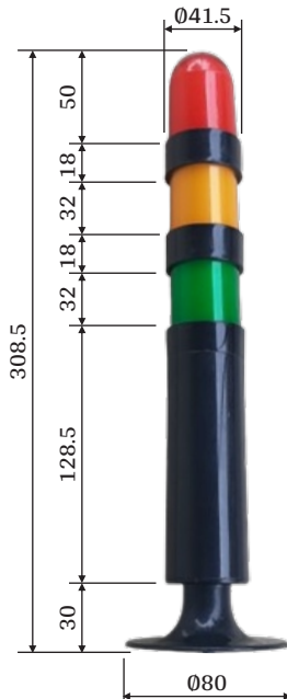
Base Mounting
